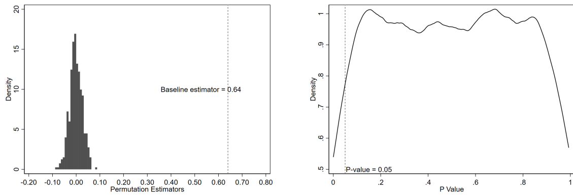
(a) Distribution of Permutation Estimators
